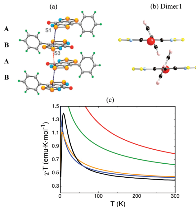
Fig. 5 (a) ab -View of the alternating ABAB \pi -stacks of PhBBO with intra-stacks S3...S1 contacts d_1 = 3.68 Å (in black) and d_2 = 3.81 Å (in red) along the a -axis ( \pi -stacking axis). (b) ac -View of Dimer1 along the a -axis ( \pi -stacking axis). (c) Magnetic susceptibility as a function of temperature using J_{AB} calculated at unrestricted B3LYP (in red), CAM-B3LYP (in green), CASSCF(14,14) (in blue) and RASSCF(38,2,2;16,6,4) (in orange). Note that the line in black corresponds to experimental data. 22
