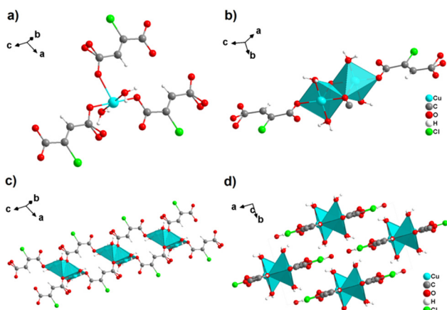
Fig. 43 Crystal structure of [Cu(OOC-CH=CCl-COO)(H 2 O) 2 ].H 2 O showing: (a) the coordination environment of Cu 2+ , (b) the dinuclear building unit with connecting chlorofumarate linkers, (c) one-dimensional ribbon extending along [001] and (d) the packing of ribbons viewed along [001]. Note: one oxygen atom of the carboxylate group neighbouring the CH moiety is disordered over two (split) positions. Graphics redrawn from the cif file (CSD-Refcode LEHJIS). 133
