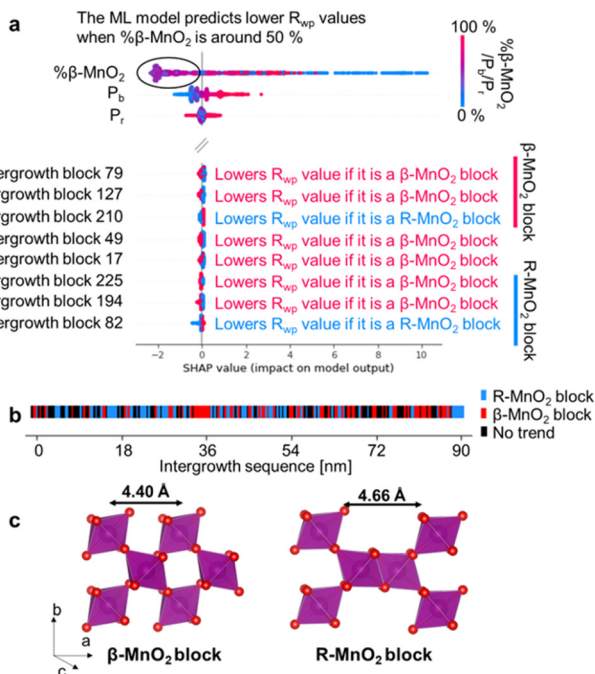
Fig. 7 Summary of the ML-MotEx analysis of the PDF data measured at sample 2. Violin plot of the SHAP values obtained in the analysis of the PDF data measured on sample 2, showing preferable % \beta -MnO 2 , P_b and P_r values and if intergrowth blocks in the starting model are favorable rather as a \beta - or R-MnO 2 block for the fit quality. (a) Each block in the supercell is colored with respect to the results from the ML-MotEx analysis. If ML-MotEx prefers the block to be R-MnO 2 , it is colored blue, if ML-MotEx does not differentiate between the blocks, it is colored black and if ML-MotEx prefers \beta -MnO 2 it is colored red. (b) Representation of a \beta -MnO 2 and of a R-MnO 2 block (c).
