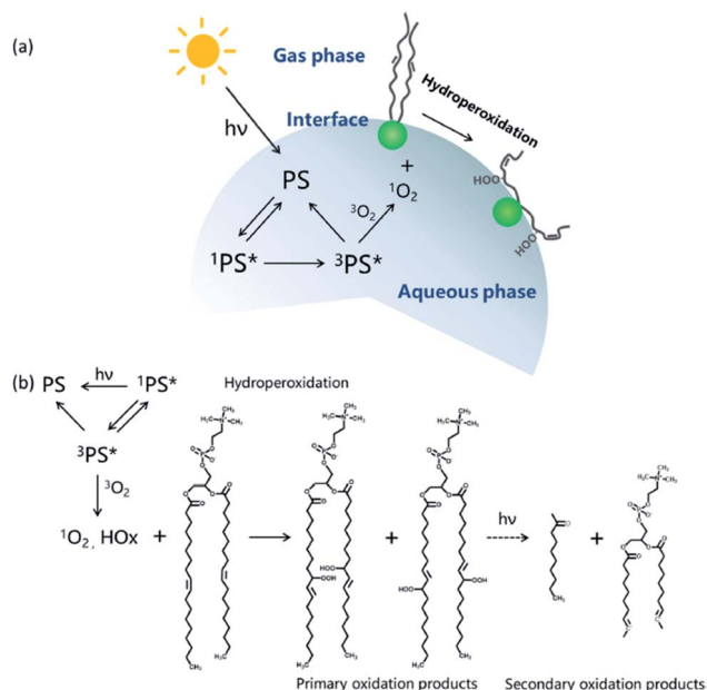
Fig. 20 (a) Cartoon and (b) products of photochemical reactions involving the lipid DOPC and photosensitizers (PS) at the air–water interface. Reprinted from ref. 440 under a CC BY 4.0 License ( https://creativecommons.org/licenses/by/4.0/ ).
