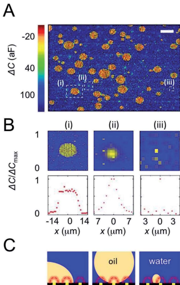
Fig. 2 (A) Capacitance image obtained with a chip incubated for 1 min in an oDCB emulsion. Each pixel in this image represents one separately addressable electrode. The scale bar represents 20 μm. (B) Capacitance image (first row) and line profile (second row) of the individual oDCB droplets shown in the dashed white rectangles in (A). The capacitance image is plotted with a color scale that maximizes the contrast between oDCB and water. The line profiles have been normalized to the maximum capacitance in the whole array while the zero is set to the minimum value of the array. (C) Cross-sectional schematic depicting the systems producing the capacitance responses shown in (B). The red dashed line schematically represents the volume of solution probed by each nanoelectrode (yellow squares). The schematic is not to scale.
