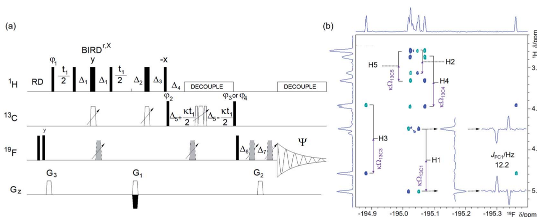
Fig. 6 (a) Pulse sequence of the (3, 2)D ^1\text{H}^{13}\text{C}^{19}\text{F} correlation experiment. For explanation of symbols used for pulses see Experimental. The NMR parameters used are given in Table S1.† The delays were as follows: d_2 = 0.25/{}^1J_{\text{HC}} ; d_3 = 0.5/{}^1J_{\text{HC}} ; d_4 = 0.25/{}^nJ_{\text{FC}} ; d_6 = \text{cnst}1/{}^1J_{\text{HC}} , where \text{cnst}1 = 0.5 for CH and 0.25 for \text{CH}_2 groups; \Delta_1 = d_3 - p14/2 ; \Delta_2 = d_2 - p14/2 - p16 - d16 ; \Delta_3 = d_2 - p14/2 - 2t_1(0) ; \Delta_4 = d_6 ; \Delta_5 = d_4 ; \Delta_6 = p16 + d16 - (2/\pi)p1 + 4 \mu\text{s} ; \Delta_7 = p16 + d16 + 4 \mu\text{s} , where p16 and d16 are the PFG length and the recovery time, respectively. The gradient strengths were as follows: G_1 = 40\% ; G_2 = 42.51\% ; G_3 = 13\% . The following phase cycling was used: \phi_1 = y, -y ; \phi_2 = 4x, 4(-x) ; \phi_3 = 2x, 2(-x) ; \phi_4 = 2y, 2(-y) ; \Psi = x, 2(-x), x, -x, 2x, -x . The echo-antiecho protocol was used with G_1 changing sign between real and imaginary increments. Phases \phi_1 and \Psi were incremented by 180^\circ together with the sign change. Two interleaved experiments were acquired applying either the \phi_3 or \phi_4 phase to the last 90^\circ ^{13}\text{C} pulse, (b) an F_1 antiphase (3, 2)D ^1\text{H}^{13}\text{C}^{19}\text{F} spectra of 1 acquired using the pulse sequence shown in (a) showing the cross peaks of the \beta -anomer of 1 . Positive and negative cross peaks are shown in blue and turquoise, respectively. The insets contain vertical and horizontal traces through the H1, F cross peaks. The ^1\text{H} chemical shift of protons directly attached to ^{13}\text{C} atoms and the associated \kappa\Omega_{13\text{C}} frequencies are indicated. Antiphase doublets in F_2 show ^nJ_{\text{FC}} coupling constants. Horizontal and vertical internal projections are shown on the top and along the left side of all spectra, respectively. The editing process that simplifies this spectrum is explained in the text and shown in Fig. S5.†
