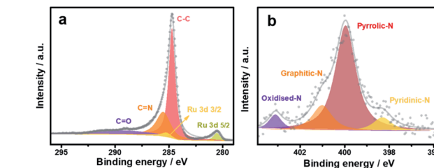
Fig. 3 (a) High-resolution XPS spectrum of C 1s + Ru 3d; (b) high-resolution XPS spectrum of N 1s.
