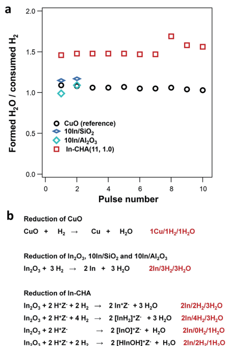
Fig. 3 (a) Determination of the formed \text{H}_2\text{O} /consumed \text{H}_2 ratio from \text{H}_2 pulses as a function of pulse number on several catalysts. (b) Stoichiometric analysis during reduction on CuO, \text{In}_2\text{O}_3 , 10In/SiO 2 , and 10In/Al 2 O 3 , and potential reactions on In-CHA catalysts.
