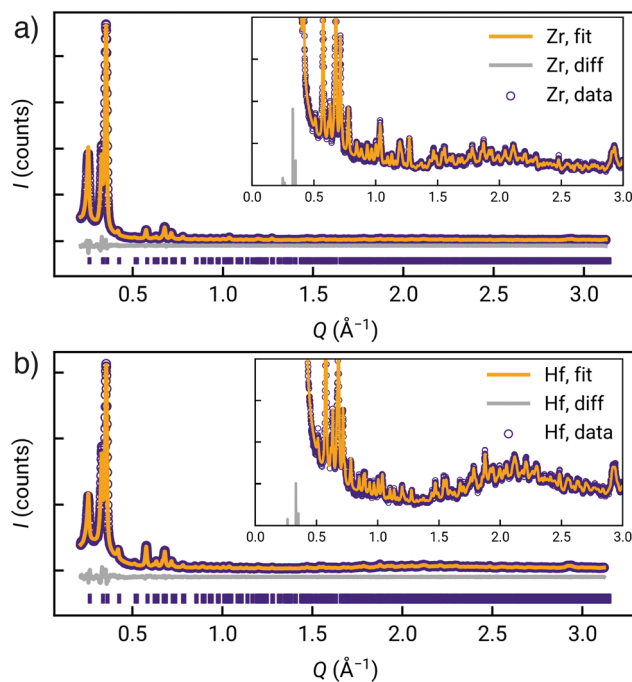
Fig. 3 Quantitative Pawley fitting (with insets to show low intensity reflections) of the powder X-ray diffractograms of a) GUF-12(Zr) and b) GUF-12(Hf).
