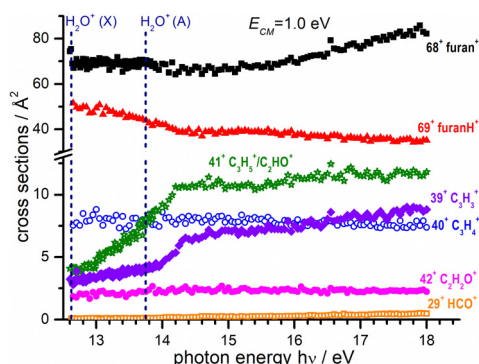
Fig. 4 Absolute reactive cross sections (in linear scale) for products m/z = 69, 68, 42, 41, 40, 39 and 29 measured at a fixed collision energy E_{CM} = 1.0 eV and as a function of photon energy. The vertical dashed lines indicate the photon energy corresponding to the opening of the ground (X) and excited electronic state A of the water radical cation. 59 Estimated uncertainties on the absolute values of the CSs are about 20% but error bars are not shown for the sake of clarity.
