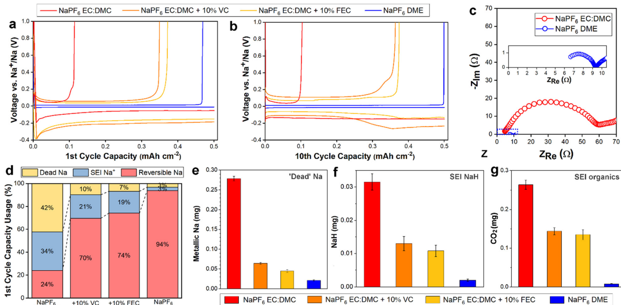
Fig. 1 Electrochemical performance comparison of sodium electrolytes with carbonate or ether solvents. Deposition capacity at 0.5 mA cm -2 for 0.5 mA h cm -2 after the (a) first and (b) tenth charge–discharge cycle. (c) EIS characterization of the ether and carbonate Na electrolytes. Magnified view of the EIS of NaPF 6 in DME shown in the insert. (d) Relative distribution of Na after the first charge–discharge cycle from titration online MS. Quantitative online MS measurements, after one cycle, of (e) 'dead' Na, (f) NaH, and (g) CO 2 , the signature of organic SEI components such as (CH 2 OCO 2 Na) 2 and NaOCO 2 R.
