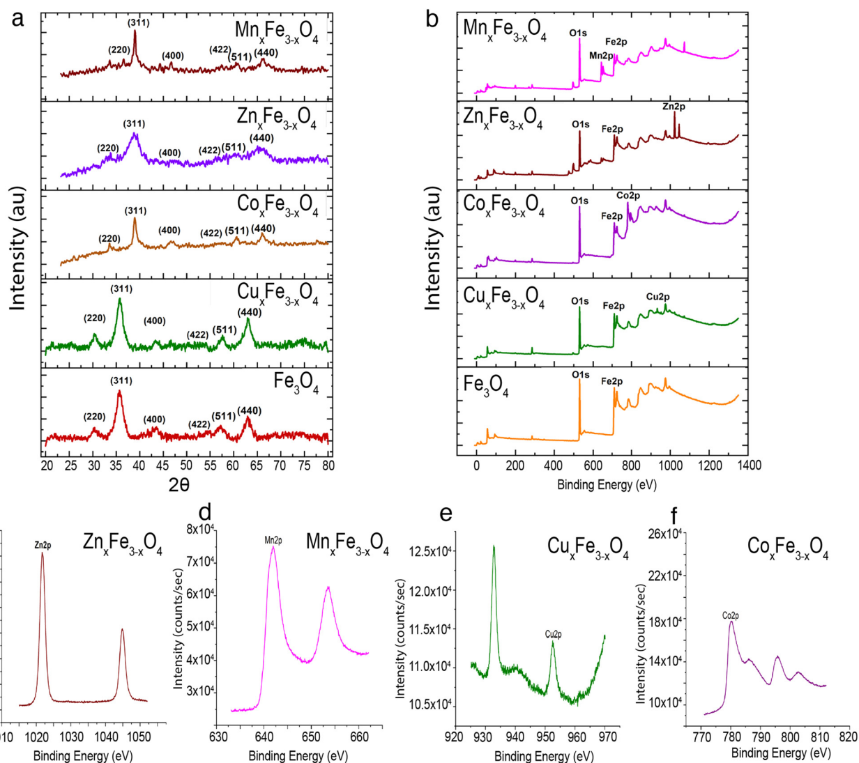
Fig. 3 Chemical characterization of various doped ferrite nanoparticles (a) XRD spectral pattern of the ferrite variants. (b) XPS spectral pattern of the ferrite variants. (c–f) Magnified XPS spectrum of individual dopants present in the ferrites to demonstrate their characteristics peaks.
