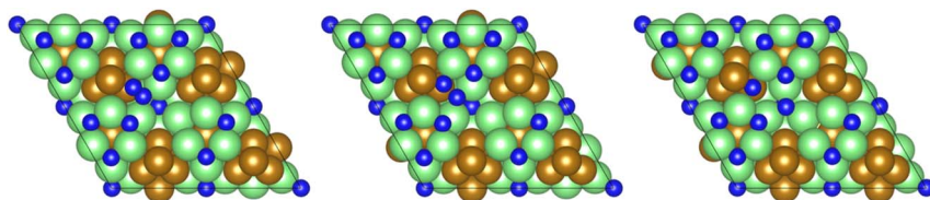
Fig. 10 Graphics illustrating the initial (left), transition (centre), and final (right) state geometries associated with \text{N}_2 dissociation (Table 3, process 2).
