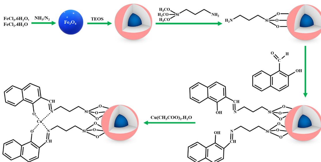
Scheme 18 Preparation of \text{Fe}_3\text{O}_4@SiO_2/\text{Schiff base}/\text{Cu} nanocatalyst.
