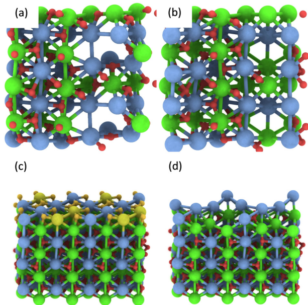
Fig. 6 The most energetically favourable structure of the \text{CaZrO}_3 bulk crystal from DFT calculations corresponding to the stoichiometry \text{Ca}_{12}\text{Zr}_{10}\text{O}_{28} (a) and \text{Ca}_{11}\text{Zr}_{12}\text{O}_{26} ( \text{CaZrO}_3 -II) (b). (001) surface of \text{CaZrO}_3 corresponding to the stoichiometry \text{Ca}_{32}\text{Zr}_{32}\text{O}_{96} (c). The yellow and orange spheres representing the Ca and O atoms were removed, creating a \text{Ca}_{29}\text{Zr}_{32}\text{O}_{69} slab corresponding to the stoichiometry of the \text{CaZrO}_3 -II sample (d). See Fig. 2 for the colour code.
