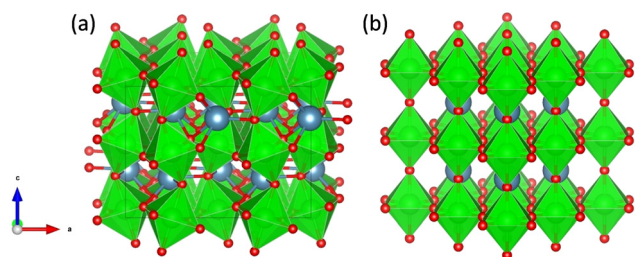
Fig. 2 Orthorhombic (a) and cubic (b) structure of \text{CaZrO}_3 . Ca, Zr and O atoms are represented by blue, green and red spheres, respectively. \text{ZrO}_6 octahedra are indicated in green.
