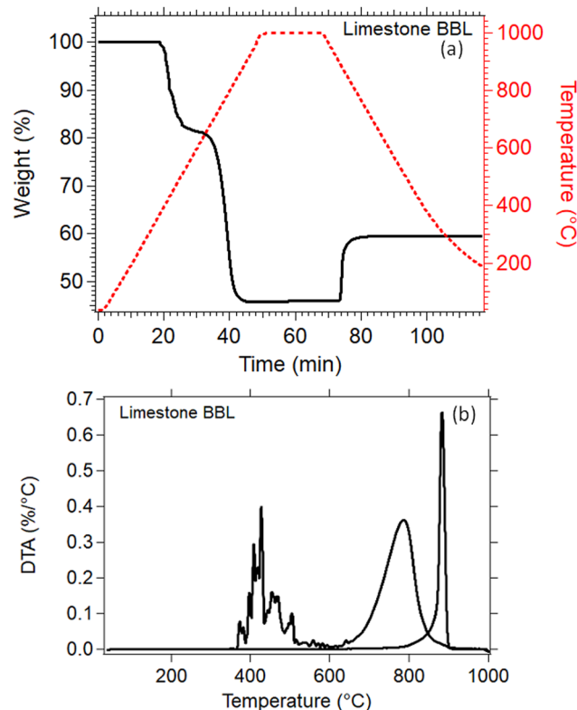
Fig. 7 (a) TGA of Lim BBL in \text{N}_2 environment up to 1000 °C (b) DTA of Lim BBL in \text{N}_2 environment up to 1000 °C.
