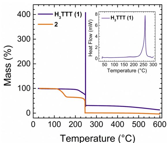
Fig. 3 Thermogravimetric analysis (TGA) of compounds 1 and 2, performed using a temperature ramp of 10 °C min −1 . The significant increase in mass percent observed at 247 °C in 1 is associated with the detonation of the material. (inset) Differential scanning calorimetry (DSC) of 1, also performed at 10 °C min −1 .
