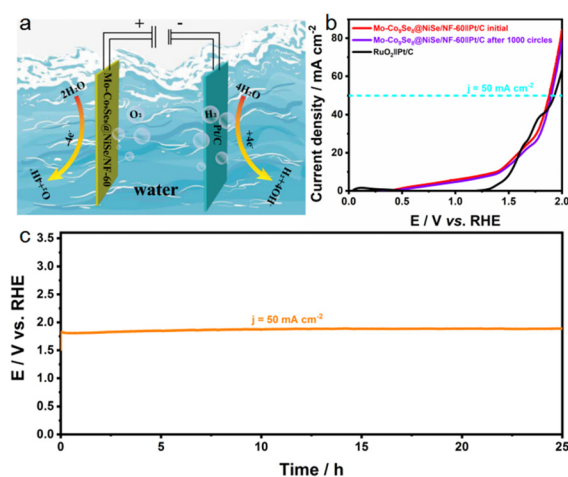
Fig. 5 (a) Schematic illustration of the electrocatalytic overall water splitting based on a Mo-Co 9 Se 8 @NiSe/NF-60||Pt/C couple. (b) LSV polarization curves of RuO 2 ||Pt/C, initial Mo-Co 9 Se 8 @NiSe/NF-60||Pt/C, and Mo-Co 9 Se 8 @NiSe/NF-60||Pt/C after 1000 circles toward water electrolysis. (c) Long-term CP curve of the Mo-Co 9 Se 8 @NiSe/NF-60||Pt/C couple at 50 mA cm -2 .
