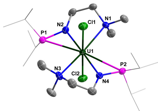
Fig. 2 Molecular structure of 1 with thermal ellipsoids at the 50% probability level. Hydrogen atoms are omitted for clarity. The \text{P}^i\text{Pr} groups on P atoms are simplified into lines. Selected bond distances (Å): \text{U1}-\text{N1} 2.698(4), \text{U1}-\text{N2} 2.249(4), \text{U1}-\text{N3} 2.691(4), \text{U1}-\text{N4} 2.248(4), \text{U1}-\text{P1} 3.0042(14), \text{U1}-\text{P2} 2.9589(14), \text{U1}-\text{Cl1} 2.6890(13), \text{U1}-\text{Cl2} 2.6856(13).
