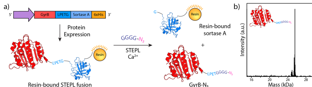
Fig. 2 Chemoenzymatic synthesis and validation of GyrB-N 3 . (a) STEPL permits one-step protein purification and C-terminal mono-functionalization of GyrB with a clickable azide handle. GyrB is appended with the genetically encoded sorting signal (LPETG) are expressed as a fusion with sortase A and a polyhistidine tag. Following chromatographic isolation, a calcium-catalyzed transpeptidation of an azide-modified polyglycine probe promotes ligation and concomitant displacement from the polyhistidine-tagged sortase. (b) Whole-protein mass spectrometry indicates that the desired GyrB-N 3 product is recovered by STEPL.
