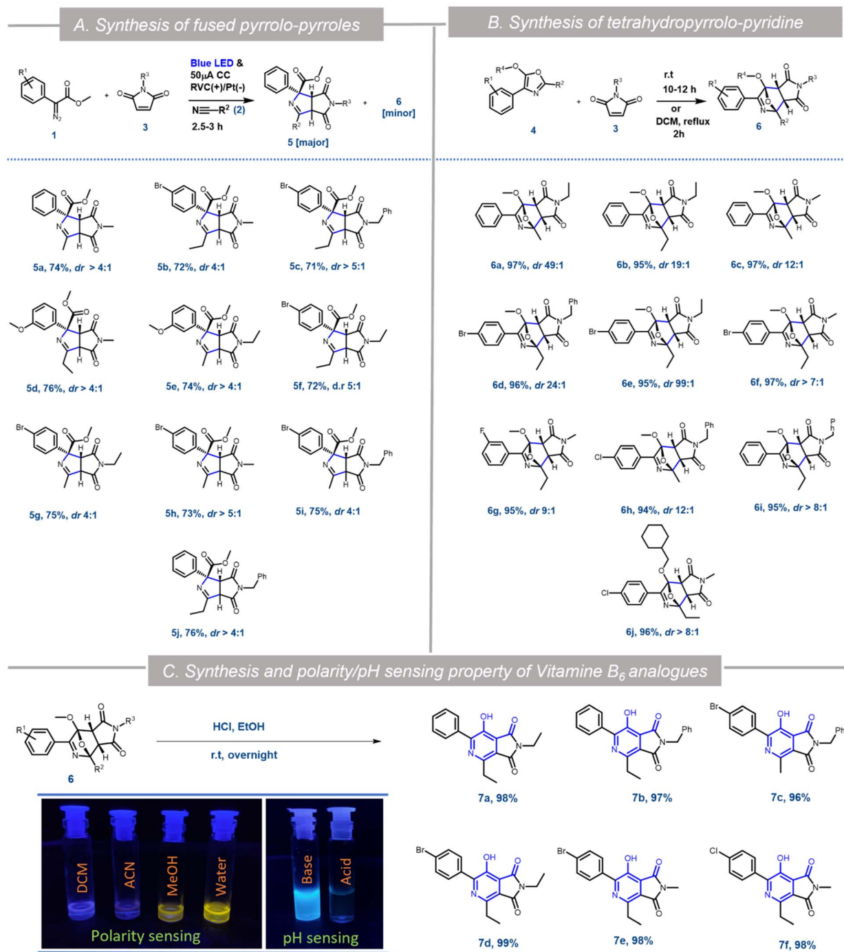
Scheme 3 Further application of the EPC reaction: (A) synthesis of pyrrolo-pyrroles through the EPC reaction, (B) synthesis of tetra-hydro-pyrrolo pyridine through the Diels–Alder reaction from oxazole; (C) synthesis and polarity and pH sensing properties of vitamin B 6 analogues [diastereomeric ratio ( dr ) determined through NMR analysis].
