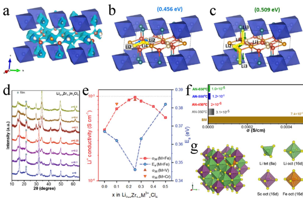
Fig. 10 (a) Li + diffusion pathways of Li 2+x Zr 1-x In x Cl 6 with an iso-surface value of \pm 0.5 v.u. Reproduced with permission. 105 Copyright 2022, Elsevier B.V. (b) Possible Li + conduction pathways in the ab -plane (b) and along the c -axis (c). Reproduced with permission. 105 Copyright 2022, Elsevier B.V. (d) XRD patterns of Li 2+x Zr 1-x In x Cl 6 . Reproduced with permission. 112 Copyright 2022, Elsevier B.V. (e) Ionic conductivity at 30 °C and activation energy for Fe 3+ /V 3+ /Cr 3+ -substituted Li 2 ZrCl 6 . Reproduced with permission. 85 Copyright 2021, Wiley-VCH. (f) Comparison of ionic conductivity between ball-milled and annealed Li 2.25 Zr 0.75 Fe 0.25 Cl 6 electrolytes. Reproduced with permission. 129 Copyright 2022, Elsevier B.V. (g) The most thermodynamically stable structure of Li 2 S 2/3 Cl 4 -0.2Fe and its components. Reproduced with permission. 95 Copyright 2023, The Royal Society of Chemistry.
