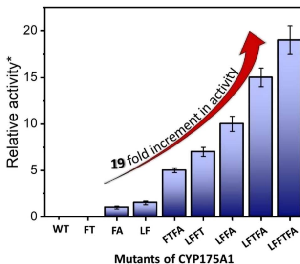
Fig. 4 Hexadecane hydroxylation activity of the mutants of CYP175A1 through the peroxide shunt pathway using \text{H}_2\text{O}_2 . *Relative fold increment in the TON with respect to the least performing FA mutant.
