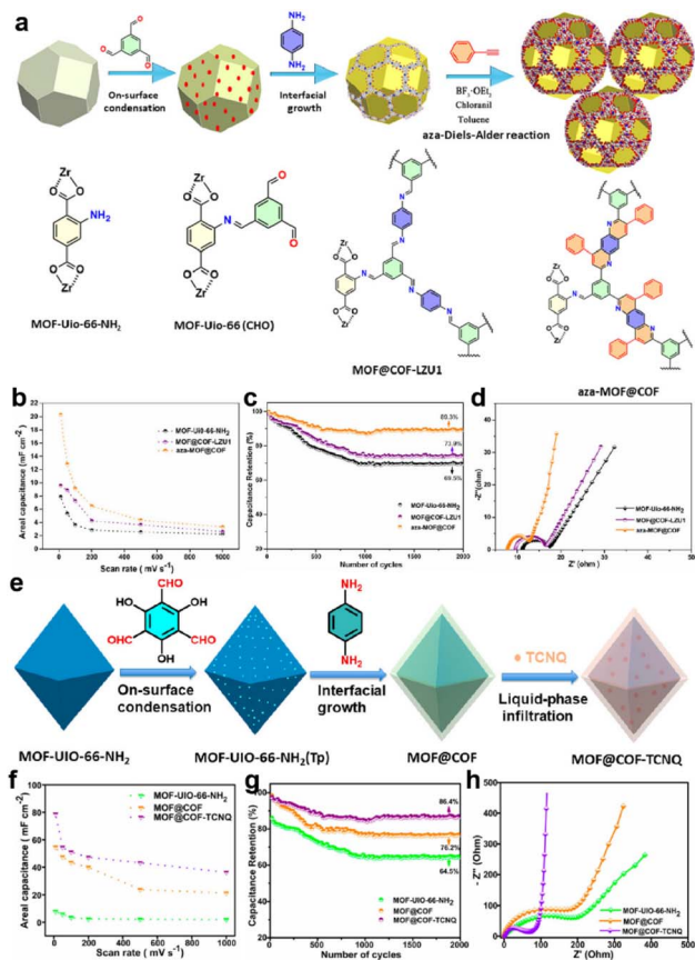
Fig. 7 (a) Illustration of the synthetic route of the MOF@COF hybrid structure. (b) Areal capacitance, (c) capacitance retention, and (d) Nyquist electrochemical impedance spectra of MOF-Uio-66-NH 2 , MOF@COF-LZU1, and MOF@COF. Reprinted from ref. 62. Copyright 2020, Wiley-VCH GmbH. (e) Schematic of the synthesis route for MOF@COF-TCNQ hybrids. (f) Areal capacitance, (g) capacitance retention, and (h) Nyquist electrochemical impedance spectra of MOF-Uio-66-NH 2 , MOF@COF, and MOF@COF-TCNQ. Reprinted from ref. 63. Copyright 2021, American Chemical Society.
