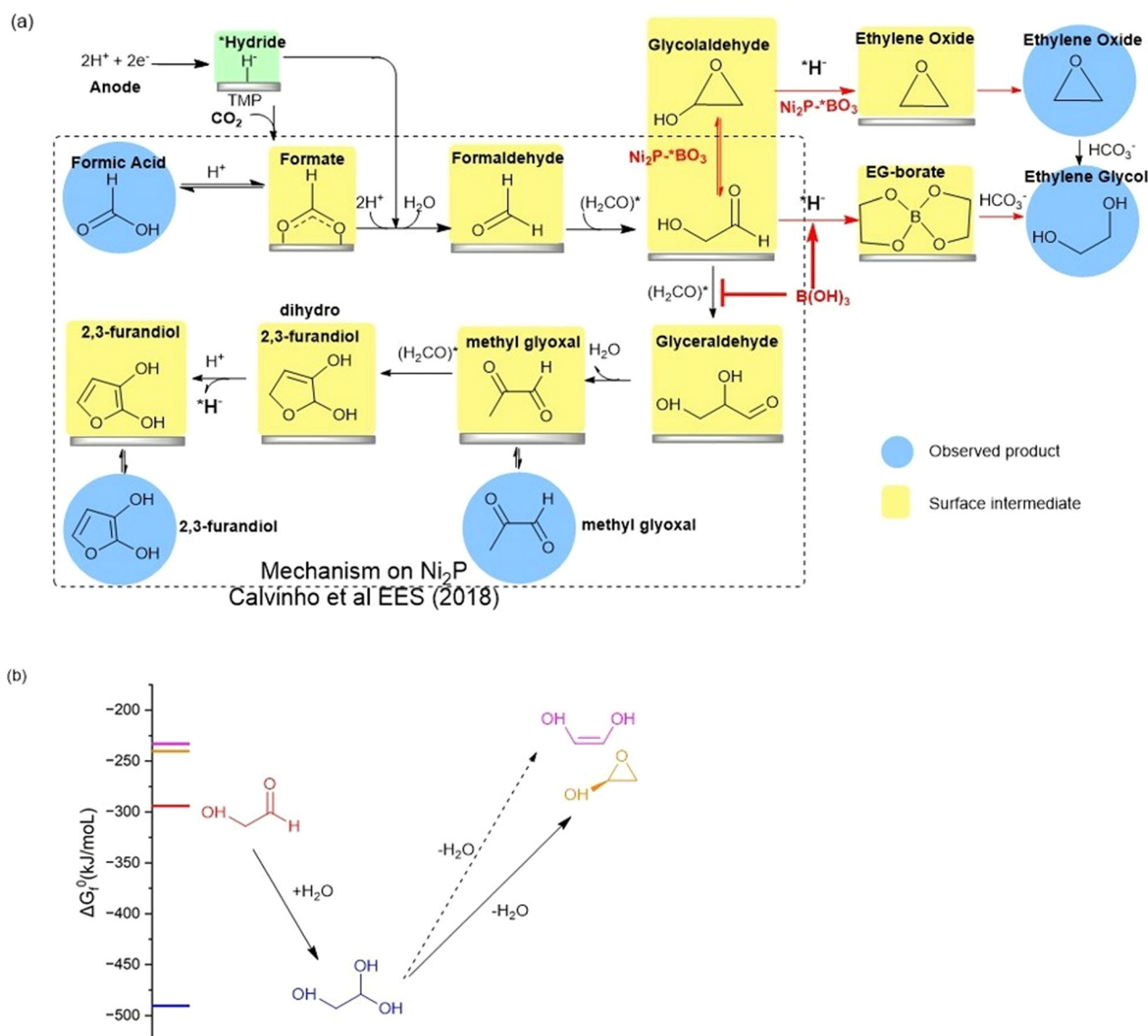
Fig. 5 (a) BLACK box: the proposed reaction mechanism for the electro catalyzed reduction of CO 2 on nickel phosphides in bicarbonate buffer as taken from Calvino et al. 1 Red arrows: the mechanism upon addition of boric acid to the electrolyte or using BO 3 *-Ni 2 P. The observed products of CO 2 RR are highlighted with blue circles, while postulated surface intermediates are highlighted in yellow boxes. (b) The chemical equilibria of glycolaldehyde in aqueous carbonate buffer showing the energetically favorable hydration to the geminal diol and dehydration by intramolecular cyclization catalyzed by carbonate. Dehydration to form the ethenediol is not expected owing to its higher energy and the mechanism requires protonation which is not possible in carbonate buffer.
