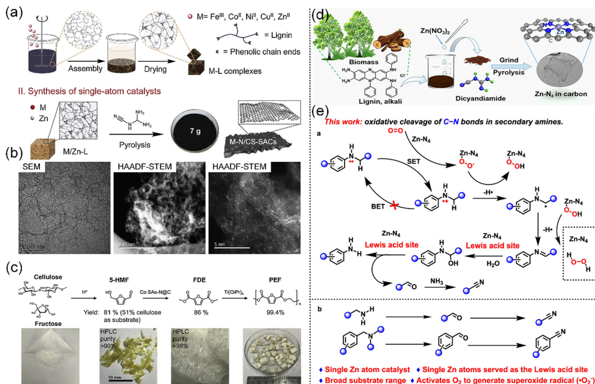
Fig. 8 (a) Strategy for the synthesis of M-N/CS-SACs. (b) TEM and HAADF-STEM images of M-N/CS-SACs. (c) Synthesis of poly(ethylene furanate) (PEF) from C 6 sugars. 5-HMF: 5-hydroxymethylfurfural and FDE: 2,5-furandicarboxylic acid dimethyl ester. (a)–(c) Reproduced with permission from ref. 59 (Copyright 2019, ScienceDirect). (d) Procedure for the preparation of the Zn-N 4 -SAC catalyst. (e) Methods for the oxidative cleavage of C–N bonds in N -alkylamines in this work. (d) and (e) Reproduced with permission from ref. 173 (Copyright 2023, the American Chemical Society).
