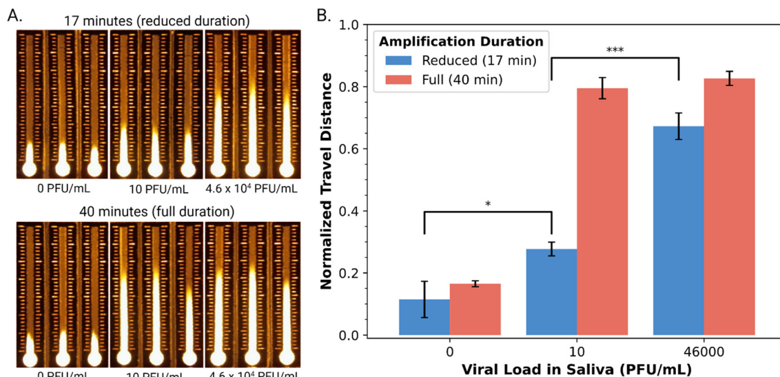
Fig. 4 DBD analysis of amplified viral RNA extracted from human saliva spiked with SARS-CoV-2. A. Representative fluorescent images of DBD substrates after exposure to amplified viral RNA extracted from three (spiked) viral loads in saliva (0-blank, 10-low, 4.6 \times 10^4 -high PFU mL -1 ) after reduced (17 min, top) and full (40 min, bottom) duration of RT-LAMP amplification. B. Plot of normalized travel distance as a function of viral load in saliva (0, 10, 4.6 \times 10^4 PFU mL -1 ) for reduced (17 min-blue) and full (40 min-red) amplification. Error bars represent \pm 1 std. deviation of normalized travel distance for n = 3 replicates per condition; a single asterisk (*) indicates statistical significance with p < 0.05 and three asterisks (***) indicate statistical significance with p < 0.001 .
