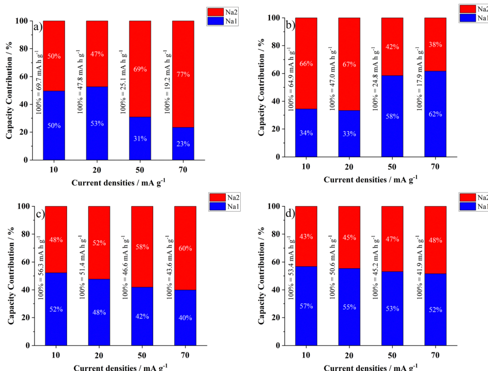
Fig. 4 Capacity contributions of (blue) \text{Na}^+_{1} and (red) \text{Na}^+_{2} to the (a) and (c) charge and (b) and (d) discharge processes of the (a) and (b) NVPF and (c) and (d) NVPF-bm electrodes.
