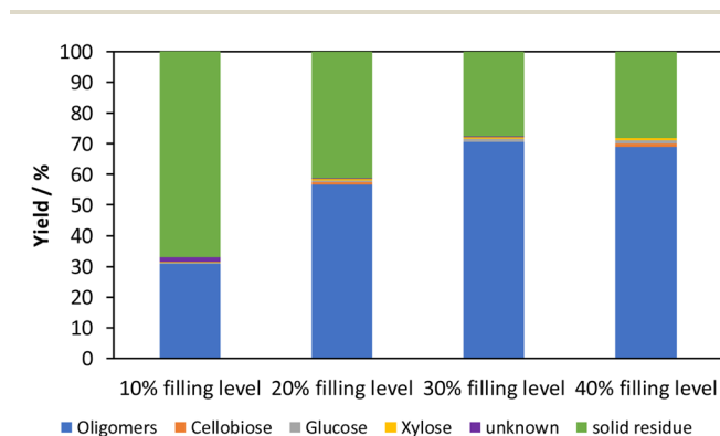
Fig. 11 Product composition after mechanocatalytic partial depolymerization by varying the filling level with tungsten carbide grinding balls. Reaction conditions: 3% acid content, 250 rpm, 85 min.
