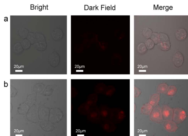
Fig. 5 Fluorescence microscopic images of HCT116 cells: (a) after treatment with 0.5 μM probe and the addition of 5 μM Hg 2+ (under red light) to probe-treated cells. (b) After treatment with 0.5 μM Au@SiO 2 probe and the addition of 5 μM Hg 2+ (under red light) to probe-treated cells.
