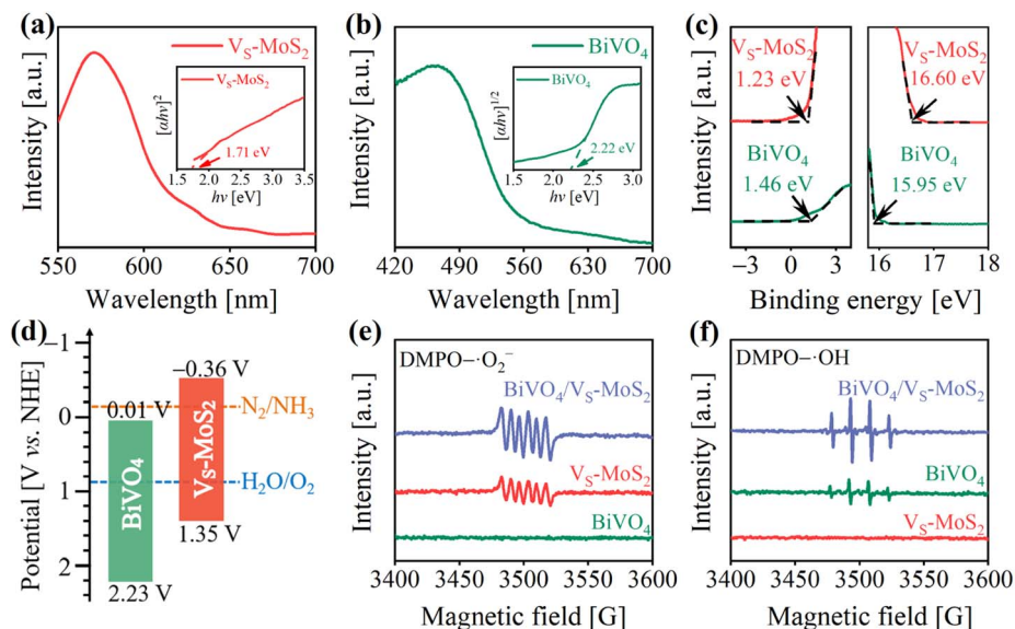
Fig. 2 (a and b) UV-vis DRS spectra of V_5-MoS_2 and BiVO_4 . The insets show the corresponding Tauc plots. (c) UPS spectra of V_5-MoS_2 and BiVO_4 . (d) Energy band structures of V_5-MoS_2 and BiVO_4 (pH = 7). EPR signals of (e) DMPO-\cdot O_2^- and (f) DMPO-\cdot OH over V_5-MoS_2 , BiVO_4 , and BiVO_4/V_5-MoS_2 under illumination.
