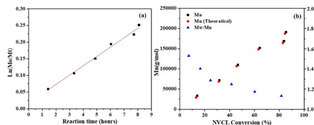
Fig. 4 (a) Semilogarithmic kinetic plot of consumption of monomer versus polymerization time. (b) Changes in \bar{D} ( M_w/M_n ) and M_n of NVCL side chains with respect to monomer conversion.
