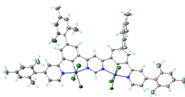
Fig. 1 The molecular structure of the dinuclear \text{Pt}(\text{IV}) complex L(\text{Pt-Cl}_3)_2 , 7 .
