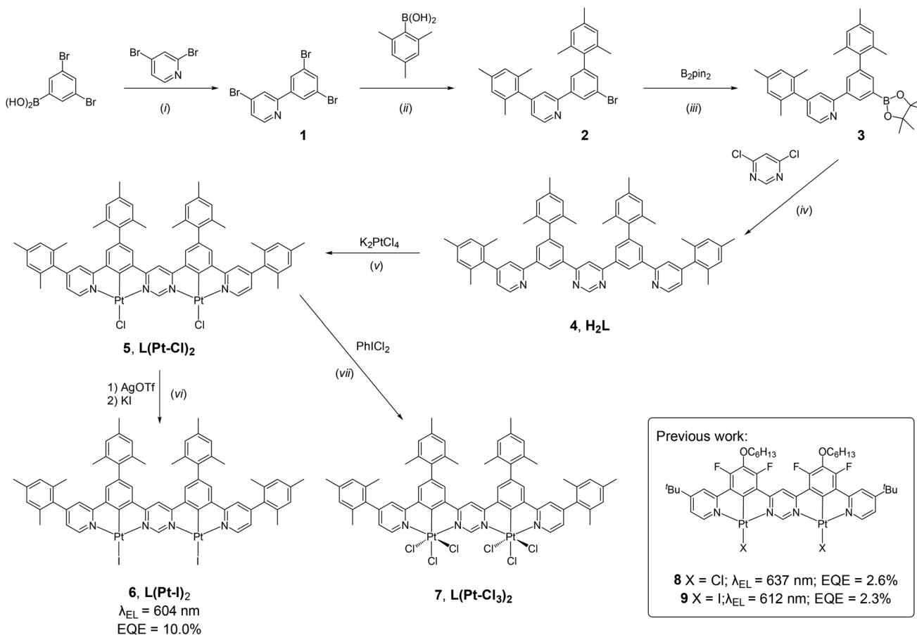
Scheme 1 Synthetic procedure for complexes 5 , 6 and 7 : (i) toluene/EtOH/ \text{H}_2\text{O} (2 : 1 : 1 v/v), \text{Pd}(\text{PPh}_3)_4 , \text{Na}_2\text{CO}_3 , 70^\circ\text{C} (2 h) \rightarrow 90^\circ\text{C} (18 h), 35%; (ii) toluene, \text{Pd}(\text{PPh}_3)_4 , \text{Cs}_2\text{CO}_3 , 90^\circ\text{C} (18 h), 67%; (iii) dioxane, \text{Pd}(\text{dppf})\text{Cl}_2 \cdot \text{CH}_2\text{Cl}_2 , KOAc, 90^\circ\text{C} (18 h); (iv) toluene, \text{Pd}(\text{PPh}_3)_4 , \text{Cs}_2\text{CO}_3 , 90^\circ\text{C} (18 h), 35%; (v) AcOH, reflux, 65%; (vi) step 1: acetone, RT (1.5 h); step 2: RT (2 h); 67%; (vii) \text{CHCl}_3 , RT (18 h), 78%. Inset: The previously studied complexes 8 and 9 incorporating a related \text{NCN-NCN} -coordinating ligand.
