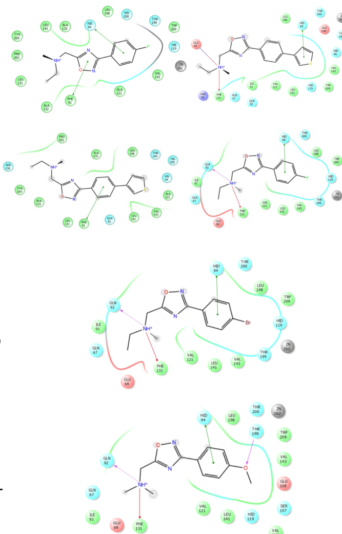
Fig. 118 Chemical structures of compounds 329–332 ; their IC 50 values against hCA-I and II along with their docking images.
