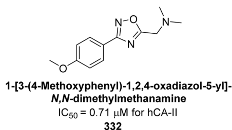
Fig. 118 Chemical structures of compounds 329–332 ; their IC 50 values against hCA-I and II along with their docking images.
