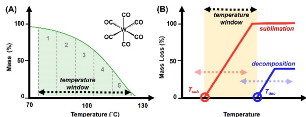
Fig. 2 (A) TGA trace of \text{W(CO)}_6 with highlighted "TGA temperature window" and illustration of sequestered zones utilized for calculation of E_a and \Delta H_{\text{sub}} . (B) General schematic to illustrate the correlation of precursor volatility and stability juxtaposed against the potential ALD temperature window.
