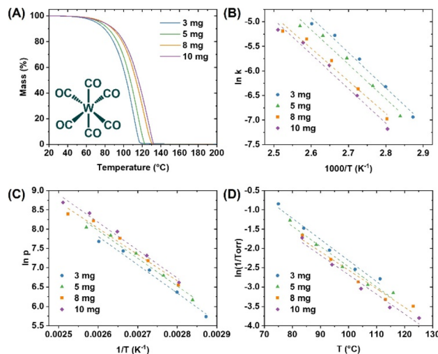
Fig. 3 Thermogravimetric analysis of \text{W(CO)}_6 : (A) precursor TG trace at a constant temperature ramp rate of 10 \text{ }^\circ\text{C min}^{-1} ; (B) the Arrhenius plot ( E_a is obtained from the slope of the curves via -E_a/R ); (C) plot of \ln p vs. 1/T , the enthalpy of sublimation is derived from the slope of the straight lines, which is equal to -\Delta H_{\text{sub}}/R ; (D) plot of \ln(1/\text{Torr}) vs. T , used to extrapolate the 1 Torr temperature. R = ideal gas constant 8.314 \text{ J K}^{-1} \text{ mol}^{-1} ( p = kPa).
