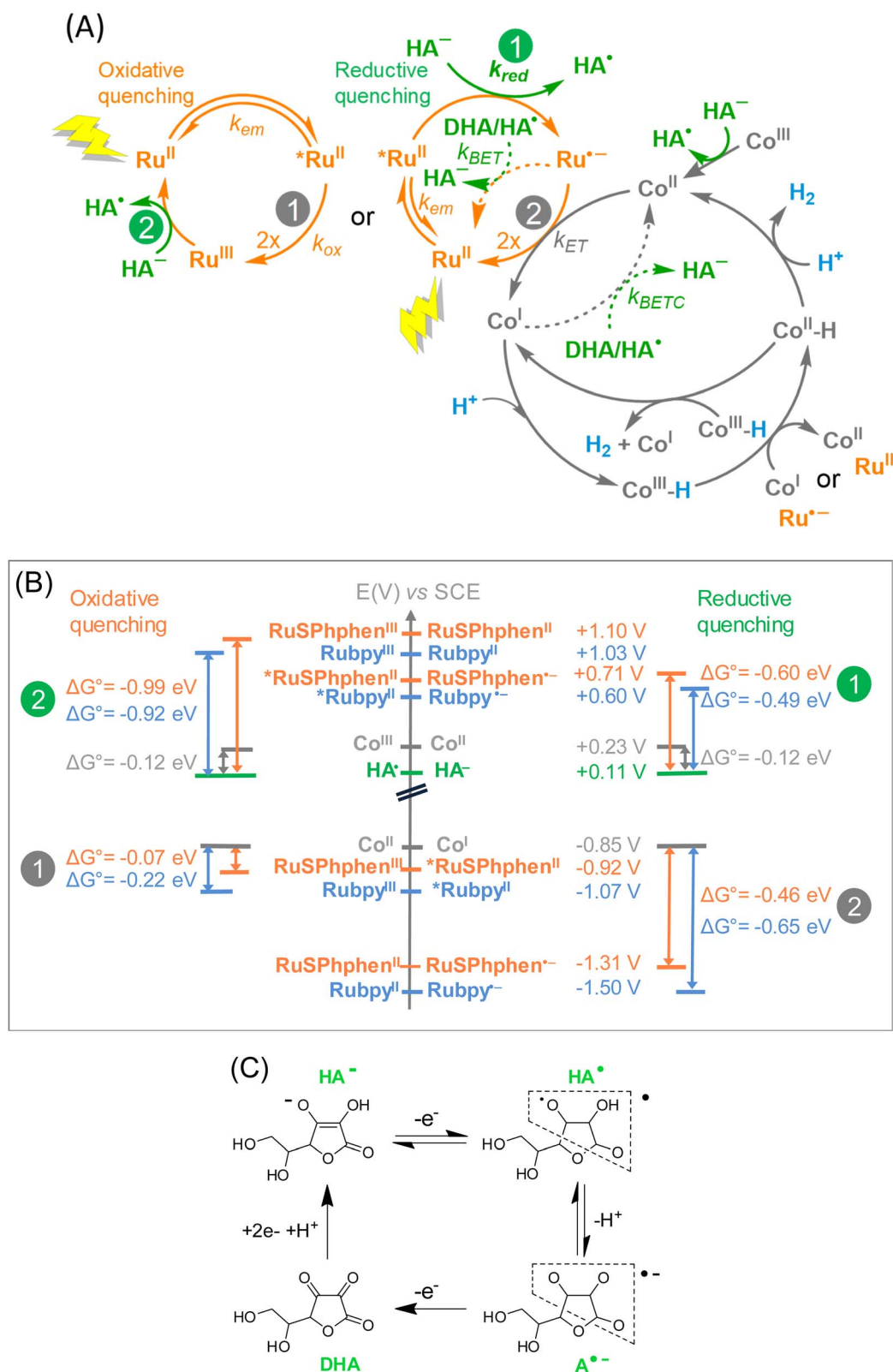
Scheme 2 (A) Possible mechanisms for the light-driven \text{H}_2 production with the system \text{Ru/Co/HA}^-/\text{H}_2\text{A} ( \text{Ru} = \text{RuSPHphen} or \text{RuSPHphen} ). (B) Diagrams of potentials referred versus SCE for the redox couples of \text{RuSPHphen} and \text{RuSPHphen} PSs at the ground and excited states, the [\text{Co}(\text{CR14})\text{Cl}_2]^+ ( \text{Co} ) catalyst, and \text{HA}^- . (C) Oxidation processes of ascorbate salt ( \text{HA}^- ) to dehydroascorbic acid (DHA) and back reduction of DHA to \text{HA}^- .
