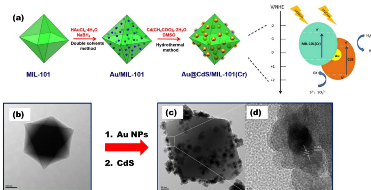
Fig. 18 (a) \text{Au@CdS/MIL-101(Cr)} synthesis route. TEM images of (b) MIL-101 and (c) \text{Au@CdS/MIL-101} . (d) HR-TEM image of \text{Au@CdS/MIL-101} . Reproduced with permission. Copyright 2016 Elsevier. 108
