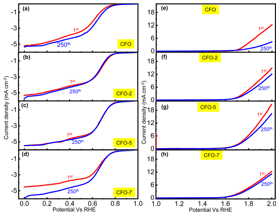
Fig. 8 (a–d) ORR cycle-life data and (e–h) OER cycle-life analysis of the CFO and the composite catalysts in 0.1 M KOH electrolyte recorded at 10 \text{ mV s}^{-1} scan rate.
