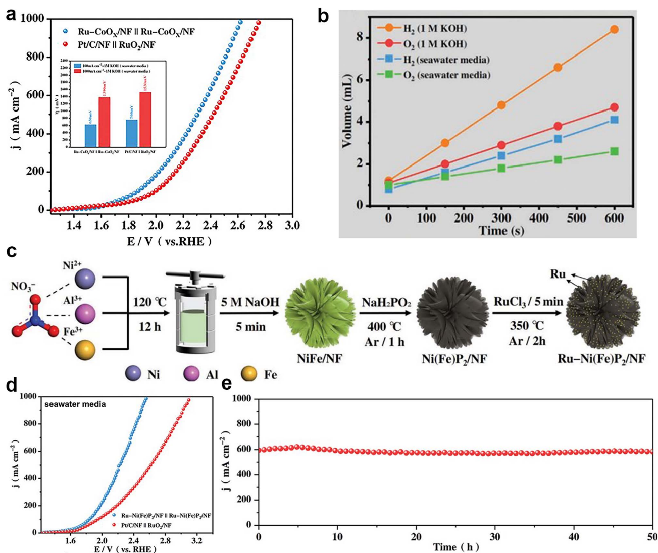
Fig. 4 (a) Polarization curves of Ru-CoO x /NF||Ru-CoO x /NF and Pt/C/NF||RuO 2 /NF toward overall water splitting in seawater media. Inset: the value of ΔE. (b) Diagram of the amount of H 2 and O 2 released over time in 1 M KOH and seawater media. Reprinted with permission. 62 Copyright 2021, Wiley-VCH. (c) Construction route of Ru-Ni(Fe)P 2 /NF. (d) Polarization curves of Ru-Ni(Fe)P 2 /NF||Ru-Ni(Fe)P 2 /NF and Pt/C/NF||RuO 2 /NF toward water splitting in seawater media. (e) 50 h constant current stability test plot of Ru-Ni(Fe)P 2 /NF in seawater media. Reprinted with permission. 63 Copyright 2023, Wiley-VCH.
