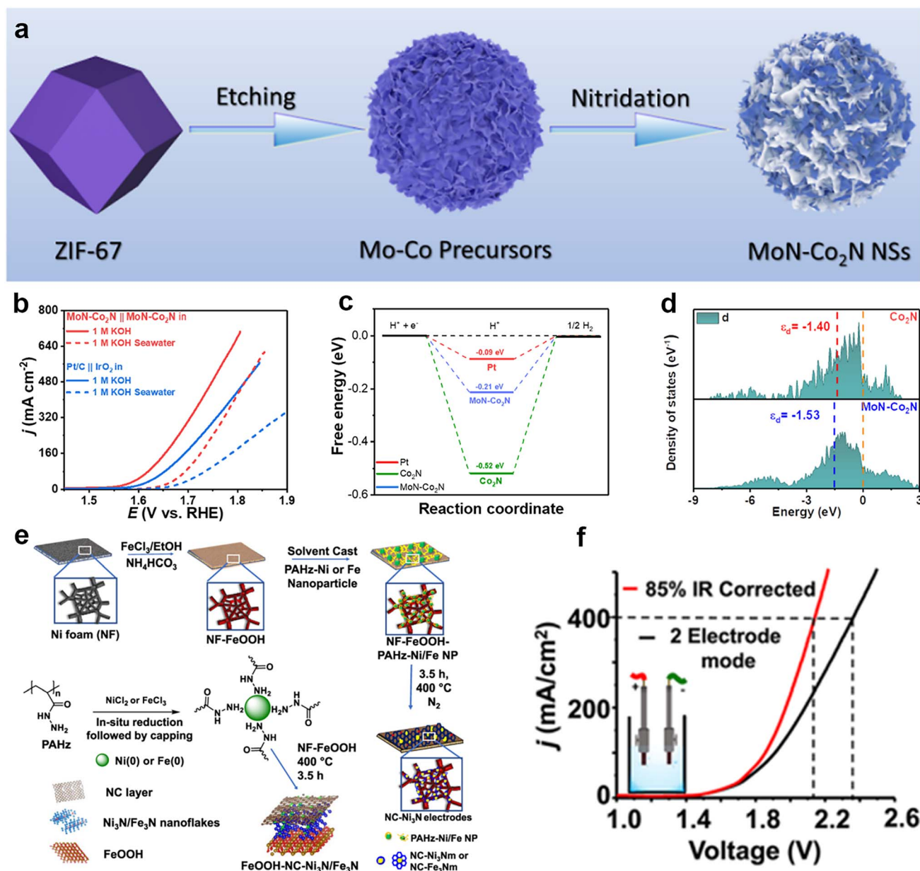
Fig. 9 (a) Schematic illustration of the synthesis of MoN-Co 2 N nanosheets. (b) Overall water/seawater splitting performance of MoN-Co 2 N/NF||MoN-Co 2 N/NF and Pt/C||IrO 2 /In pairs in 1 M KOH and 1 M KOH seawater. (c) Calculated free energy diagram of H* adsorption on the surface of Pt, Co 2 N, and MoN-Co 2 N. (d) The d-band centers of Co 3d partial DOS for Co 2 N and MoN-Co 2 N. Reprinted with permission. 88 Copyright 2022, American Chemical Society. (e) Schematics showing the FeOOH coating of the NF, followed by the in situ growth of the NC-Ni 3 N or NC-Fe 3 N nanocomposite layer and synthesis of PAHz-Ni/Fe nanoparticles, followed by NC-Ni 3 N/Fe 3 N nanocomposite. (f) IR-uncorrected and corrected LSV traces of NC-Ni 3 N 21 recorded under two-electrode mode in seawater possessing 2 M KOH. Reprinted with permission. 89 Copyright 2023, American Chemical Society.
