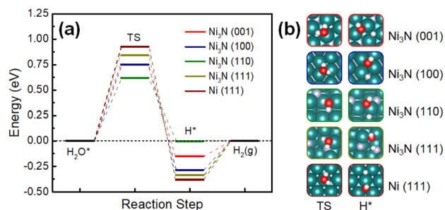
Fig. 6 (a) Calculated HER free energy pathways on \text{Ni}_3\text{N} (001), \text{Ni}_3\text{N} (100), \text{Ni}_3\text{N} (110), \text{Ni}_3\text{N} (111), and Ni (111) surfaces in alkaline media. (b) Modelled Ni-terminated \text{Ni}_3\text{N} and Ni metal surfaces at two different states [i.e., transition state (TS) and \text{H}^* -adsorbed state]. Green, blue, red, and white spheres represent Ni, N, O, and H, respectively.
