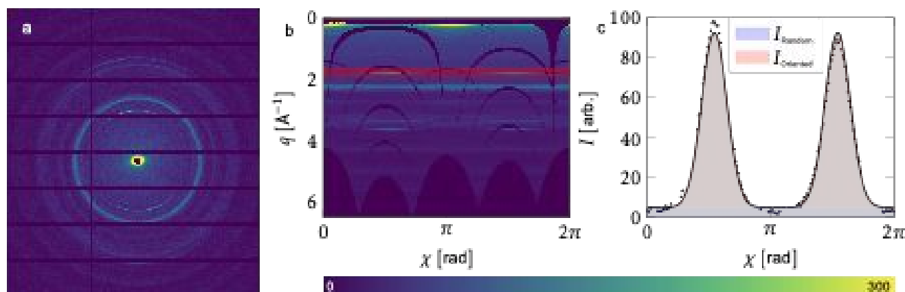
Figure 2: Orientation analysis. Raw detector frame (a). Azimuthally resolved detector frame after integration. The red box indicates the (002) peak, which shows the c -axis orientation of the apatite crystallites (b). Local background subtracted (002) orientation signal. The dots show the data, line shows fit. The position of the peak gives the orientation, the ratio I_{\text{oriented}}/(I_{\text{oriented}}+I_{\text{random}}) gives the DoO and the total signal is the sum of the red and blue areas (c).
