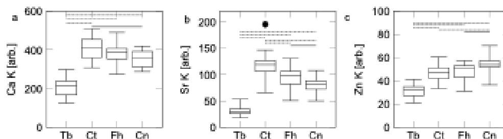
Figure 4: Statistics analysis of XRF data. Ca (a). SR (b). And Zn (c) a solid line significance level ^{*} ( p<0.05 ) whereas a dashed line signifies a difference a different significance level ^{**} ( p<0.01 ). Black dots show outliers.
