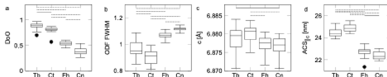
Figure 6: Statistics analysis of diffraction data. With the Degree of Orientation (DoO) mean (a). Orientation distribution function FWHM (b). Unit cell c-axis (c). Apparent crystallite size parallel to the c-axis (d). A solid line shows a significance level ^{*}(p < 0.05) whereas a dashed line shows a significance level of ^{**}(p < 0.01) . Black dots indicate outliers
