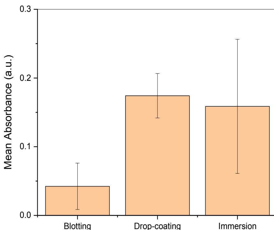
Figure 1: Mean absorbance signal at 1620 cm -1 (wave number), indicative of the presence of the \beta -sheet conformation, assessed by Fourier Transform Infrared Spectroscopy (FTIR) using three different deposition methods: blotting, drop-coating, and immersion. The error bars represent the standard deviation (SD).
