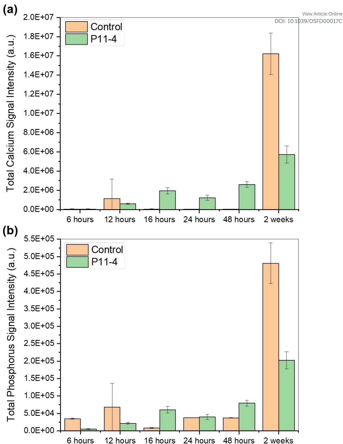
Figure 6: Mean total signal intensity of (a) calcium and (b) phosphorus with time (6 hours, 12 hours, 16 hours, 24 hours, 48 hours and 2 weeks) comparing the control to the SiN windows with deposited P 11-4 . The 400 \mu\text{m} x 400 \mu\text{m} map was split into eight regions, from which the calcium and phosphorus signals intensity was calculated to calculate the mean total signal intensity value of calcium and phosphorus. The error bars indicate the standard deviation of values.
