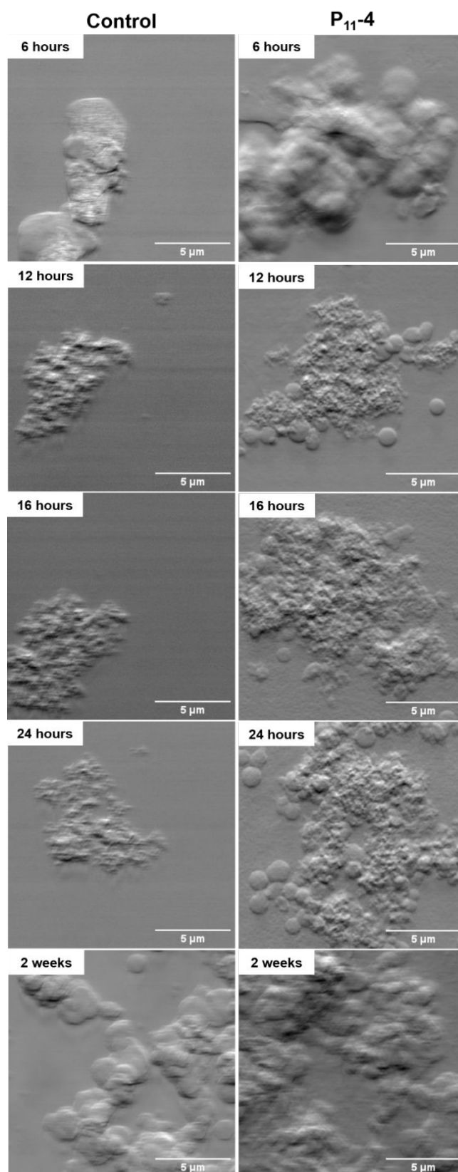
Figure 2: Typical Differential Phase Contrast (DPC) images of SiN windows with deposited P_{11-4} and without (control) mapped on the I14 beamline at different time points, depicting the morphology of the crystals formed after immersion in mineralising solution. The area shown is 15\ \mu\text{m} \times 15\ \mu\text{m} , with a step size of 50\ \text{nm} .
