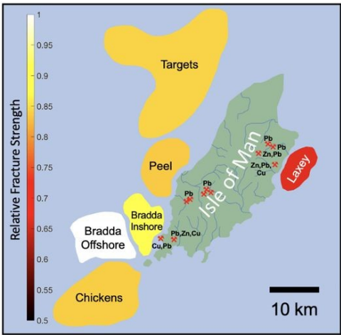
Figure 2 : Map of the relative mean fracture strength observed for Pecten maximus around the Isle of Man with the value for Bradda Offshore used to normalize the values for all other sites. Shells were collected from six sites around the Isle of Man in 2004. The color code indicates the value for the relative fracture strength. Laxey is the contaminated site, all the others are controls ( n = 20 per site, 120 in total). The value for the Laxey site is 0.66 whereas the values for the other sites are all above 0.83. Red symbols assign major historical mining sites for zinc, lead and copper ores with the order of importance indicated by their sequence position. [10]
