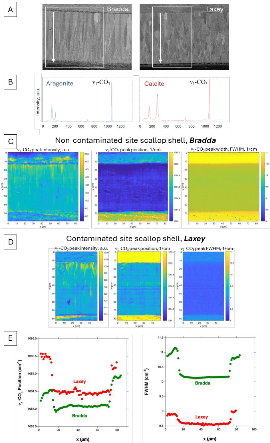
Figure 8: (A) BSE images of a sample from non-contaminated (Bradda) and contaminated (Laxey) sites; (B) Raman spectra taken from the myostracum and foliated regions of the Bradda sample, (C) \nu_1 -CO 3 Raman maps evaluating peak intensity, position and full width at half maximum of the Bradda and (D) and Laxey samples, (E) Comparison of line profiles from top to bottom of the \nu_1 -CO 3 Raman position and full width at half maximum for Bradda and Laxey samples.
