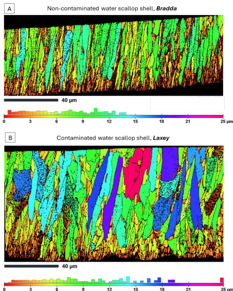
Figure 7 : EBSD grains maps with a color scale according to grain size (longest dimension) in the myostracum.
