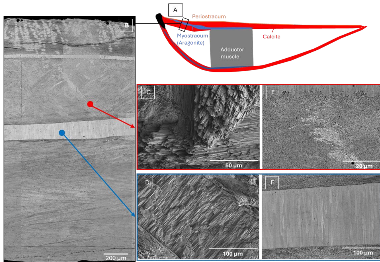
Figure 1 : (A) Schematic longitudinal section of a king scallop ( Pecten maximus ) shell, both valves. Of the organic parts only the adductor muscle is indicated showing its attachment to the shell via an aragonitic calcium carbonate layer. (B) Backscattered electrons stitched SEM images of a king scallop sample from a non-contaminated area after surface polishing. SEM images of king scallop in calcite (red) area: (C) Secondary electron image of calcite foliated grains on laser cut surface and (E) backscattered electron image of calcite foliated grain after surface polishing. SEM images of king scallop myostracum aragonite prismatic layer (blue) area: (D) Secondary electron image of myostracum layer on laser cut surface and (F) backscattered electron image of myostracum layer after surface polishing.
