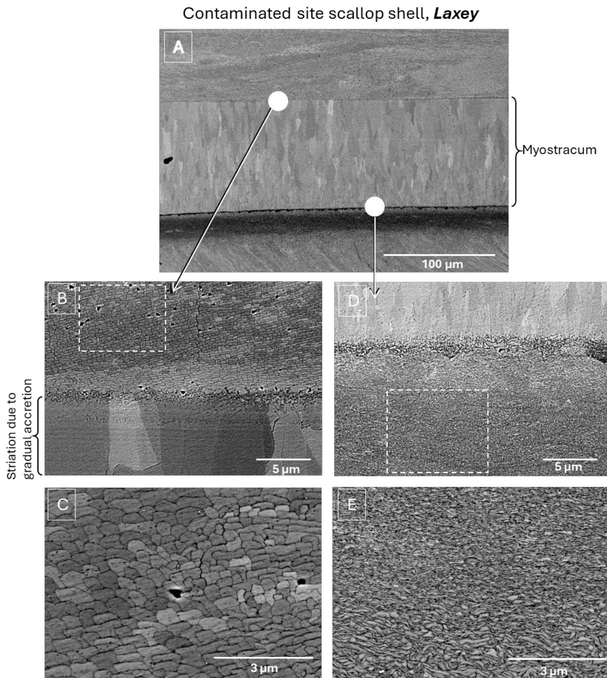
Figure 5 : BSE micrographs of the myostracum region for the scallop shell collected in the contaminated Laxey area. (A) provide a general view of the region of interest. (B) display the upper boundaries between the myostracum and the shell bulk. (C) show the microstructures of the scallop in the region at the top of the myostracum. (D) illustrate the lower boundaries between the myostracum and the shell bulk. (E) present the microstructures of the shell in the region below the myostracum.
