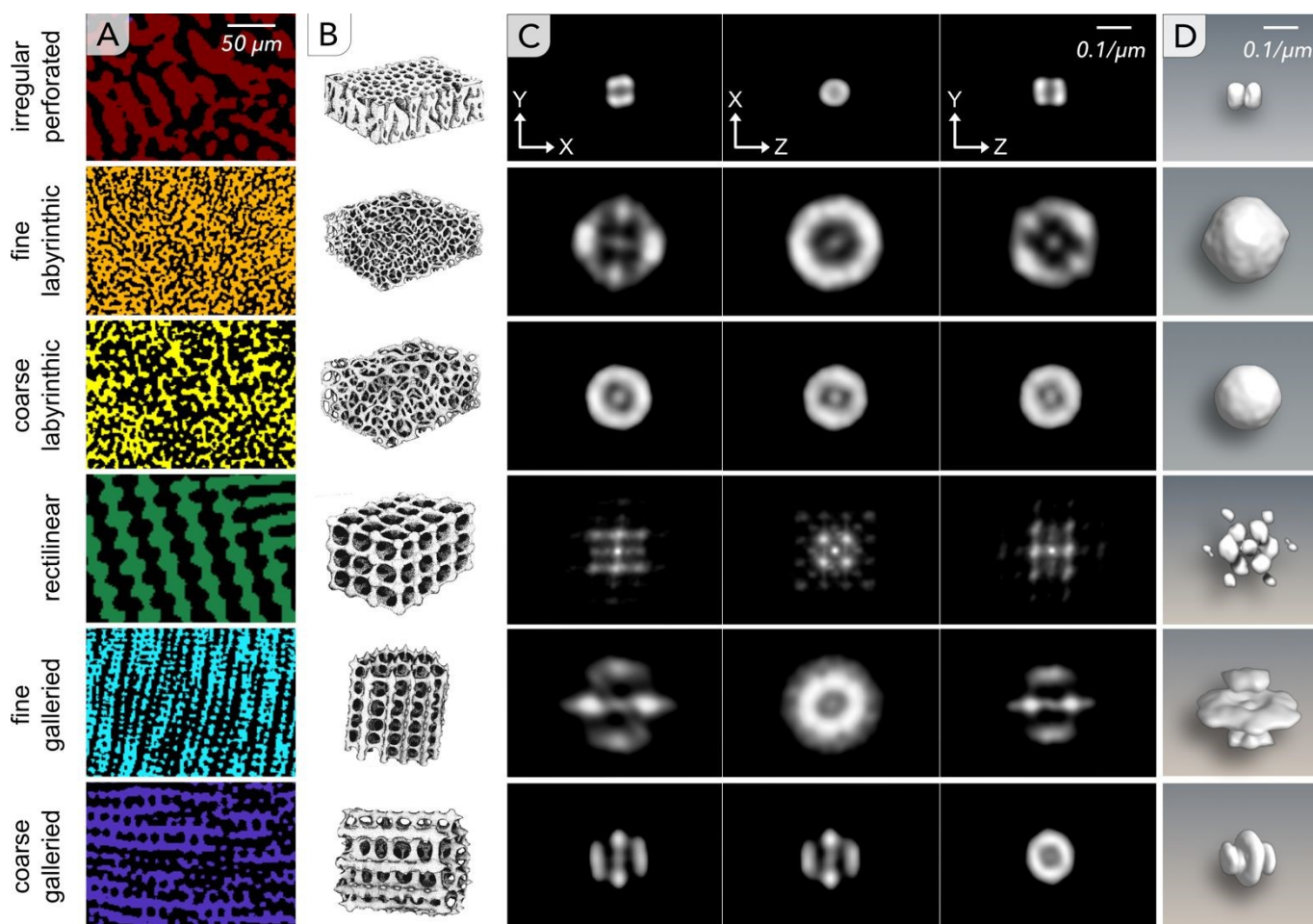
Figure 4. A) Virtual CT slices through representative sub-volumes for each of the identified stereom types. B) Drawings [Smith 1980, reproduced with permission] depicting the three dimensional appearance of the different stereom types. C) Virtual sections through the power spectra of each stereom type. The section planes are aligned normal the principal directions of the power spectra. D) Renderings of isosurfaces of power spectra for each stereom type.
