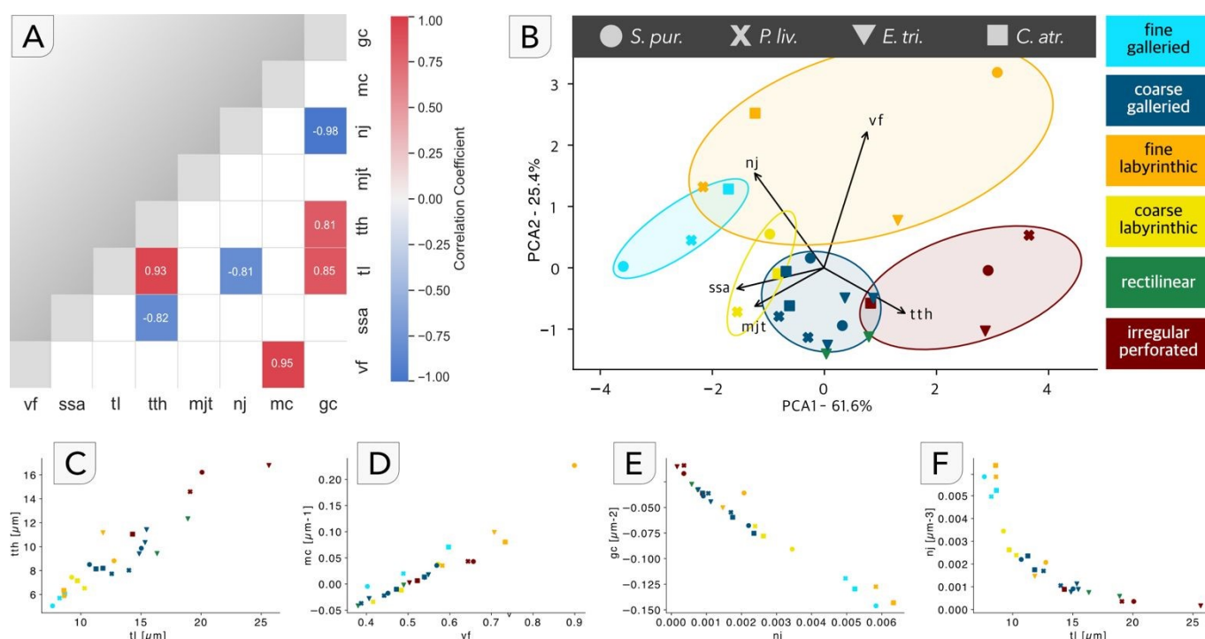
Figure 5. A) Matrix of correlation pairwise correlation coefficients for descriptors of the 6 major stereom subtypes found in the coronal plates of four species of sea urchins. vf: mineral volume fraction [a.u.]; ssa: specific surface area [ \text{m}^2 \cdot \text{cm}^{-3} ]; tth: mean trabecular thickness [ \mu\text{m} ]; tl: mean trabecular length [ \mu\text{m} ]; mjt: mean joint type as defined in the scan library; nj: number density of trabecular junctions [ \mu\text{m}^{-3} ]; mc: mean curvature [ \mu\text{m}^{-1} ]; gc: gaussian curvature [ \mu\text{m}^{-2} ]. B) Biplot of principle component analysis of morphometric descriptors for 6 major stereom subtypes (cyan: fine galleried; blue: coarse galleried; orange: fine labyrinthic; yellow: coarse labyrinthic; green: rectilinear; red: irregular perforated) found in the coronal plates of four species of sea urchins (circle: S. pur. ; cross: P. liv. ; triangle: E. tri. ; square: C. atr. ). Loadings for the descriptors vf, ssa, tth, mjt, and nj are indicated (black arrows). The confidence ellipses are drawn with radii of 1.6 standard deviations and are shaded according to the color of the stereom subtype they represent. The associated scree plot is presented in Fig. SI 3 C-F) Scatterplots of the strongly correlated descriptor pairs trabecular thickness and length (C), mean curvature and volume fraction (D), gaussian curvature and number density of trabecular junctions (E), and number density of trabecular junctions and mean trabecular length (F).
