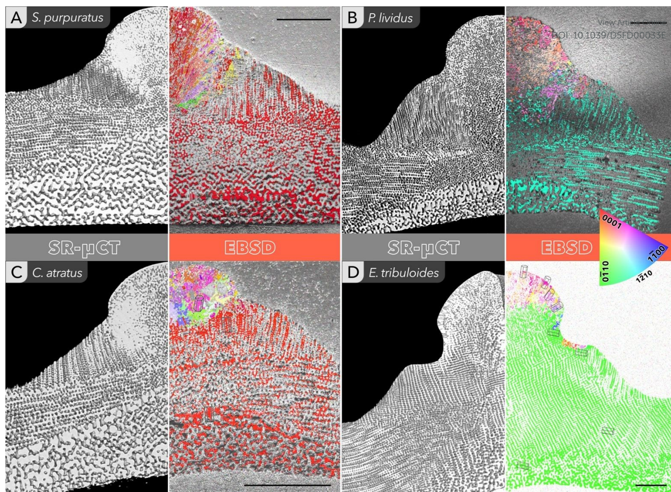
Figure 2. A-D, (left image) Rendering of virtual section through binarized SR-μCT reconstruction of interambulacral test plate of Strongylocentrotus purpuratus (A), Paracentrotus lividus (B), Colobocentrotus atratus (C) and Eucidaris tribuloides (D). Note that only the left half of each section is shown. Right image) Crystallographic orientation maps superimposed on backscattered electron images of ground-and-polished sections of interambulacral test plates. For the color key, refer to the inverse pole figure of calcite (inset). The reference direction is aligned with the y-direction of the map. Scale bars: 500μm.
