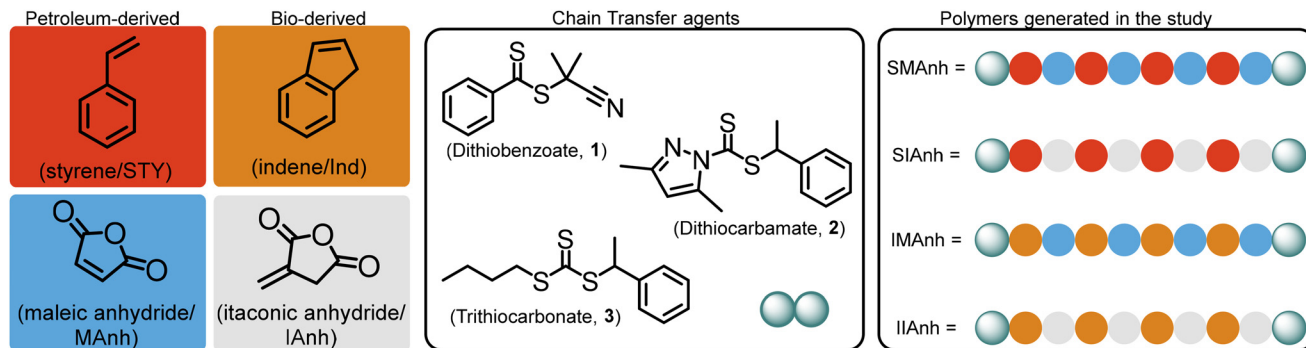
Fig. 1 Copolymers synthesized using styrene (STY), indene (Ind), maleic anhydride (MANh), and itaconic anhydride (IANh). poly(styrene- alt -maleic anhydride) (SMAAnh), poly(styrene- alt -itaconic anhydride) (SIAnh), poly(indene- alt -itaconic anhydride) (IIAAnh), poly(indene- alt -maleic anhydride) (IMAnh).
