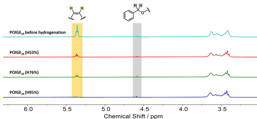
Fig. 5 1 H NMR spectra of POIGE 25 and the respective hydrogenated polymers (400 MHz, CDCl 3 ). The value of H denotes the degree of hydrogenation. The intensity was locally normalized to the initiator benzyl group (gray).
