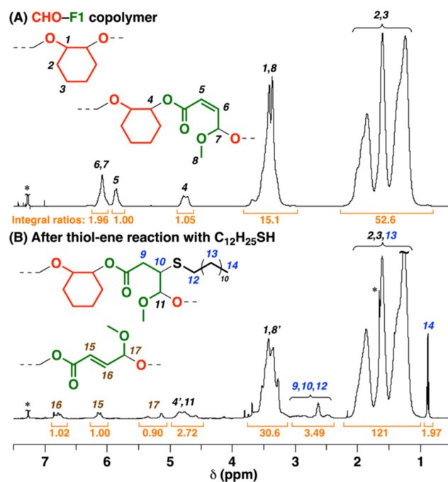
Fig. 6 1 H NMR spectra of (A) CHO-F1 copolymer (obtained under similar conditions to those for entry 1 in Table 3; the average number of CHO/F1 units per block = 6.6/1.0) and (B) the product obtained by the thiol-ene reaction of the copolymer ([double bonds in copolymer] 0 = 0.062 M, [C 12 H 25 SH] 0 = 0.31 M, [AIBN] 0 = 0.031 M, in toluene at 80 °C, 24 h). See Fig. S22† for the MWD curves. * CHCl 3 or water.
