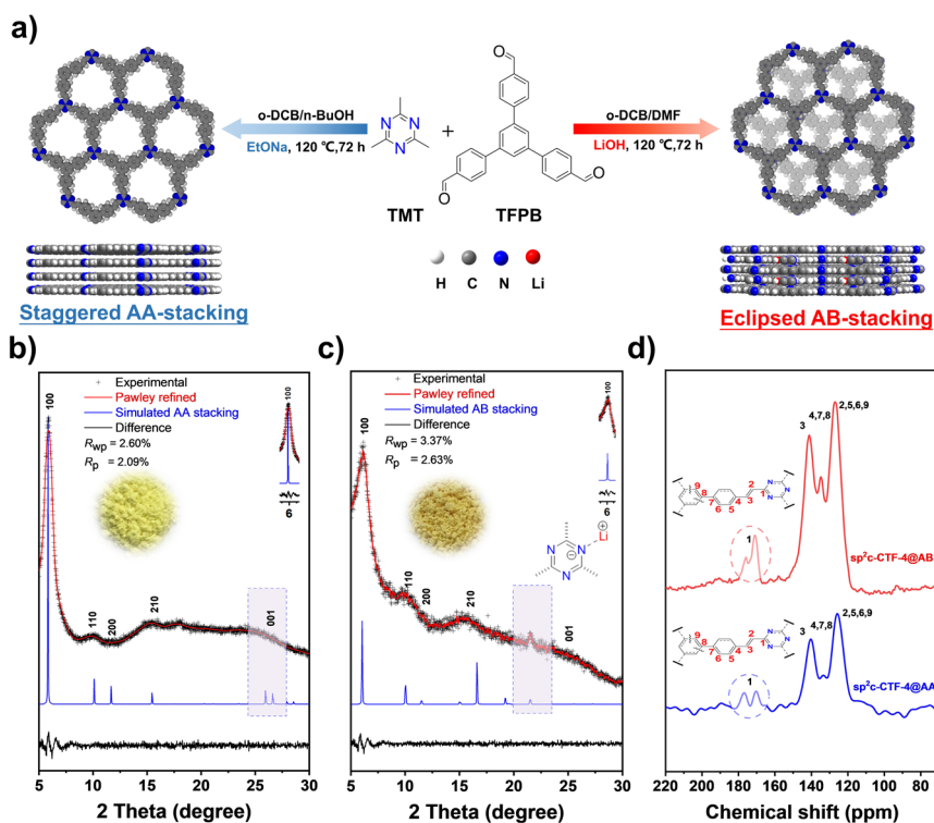
Fig. 1 (a) Schematic diagram for the synthesis of \text{sp}^2\text{c} -CTF-4 and views of the corresponding refined 2D crystal structure; PXRD patterns of (b) \text{sp}^2\text{c} -CTF-4@AA and (c) \text{sp}^2\text{c} -CTF-4@AB; comparison between the experimental (black cross) and Pawley refined (red line) profiles, the simulated patterns for AA and AB stacking mode (blue line); (d) ^{13}\text{C} CP/MAS solid-state NMR spectra of \text{sp}^2\text{c} -CTF-4@AA and \text{sp}^2\text{c} -CTF-4@AB.
