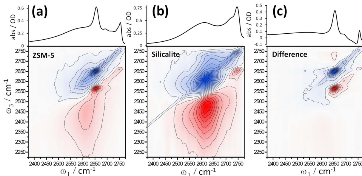
Fig. 3 IR absorption and 2D-IR spectra of deuterated pellets of ZSM-5 (a) and silicalite (b) held at \sim 210 °C between CaF 2 plates in an atmosphere of dry N 2 . Crossed polarisation \langle \text{XYYY} \rangle and a waiting time of t_2 = 1 ps were used. Subtractions of the silicalite from the ZSM-5 2D-IR and IR spectra are shown in (c). The IR absorption spectra are baseline corrected using a 'best-guess' curve for the scatter contribution. A scale factor of \sim 0.5 applied to the silicalite spectrum best subtracts the nest band in the ZSM-5 2D-IR and IR spectra.
