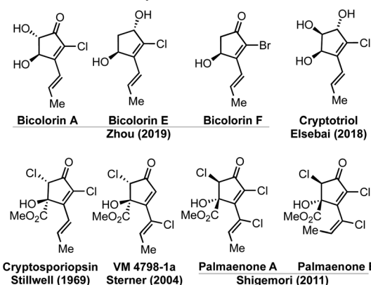
Fig. 1 Cyclohelminthol I–IV and related natural products. Name and year refer to isolation study.
