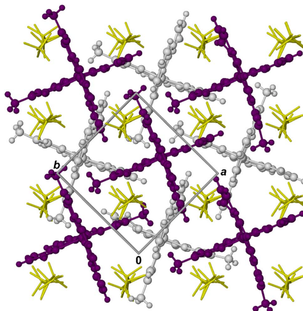
Fig. 2 Packing diagram for 1[\text{ClO}_4]_2 at 100 K viewed parallel to the [001] vector, with a random distribution of cation orientations. Alternate cation layers in the lattice are coloured white and purple, while the \text{ClO}_4^- ions (yellow) are de-emphasised for clarity.
